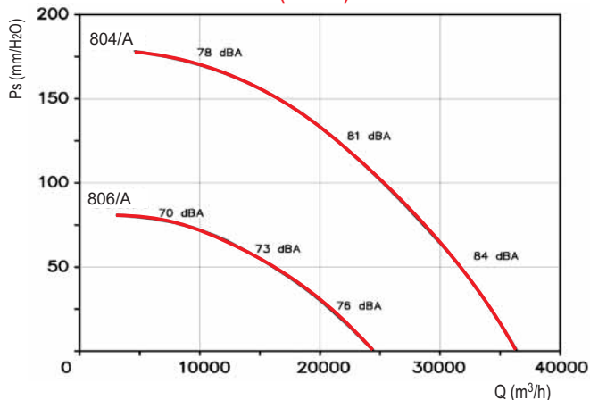
ROOF-HP 800/A (F400)
