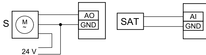
Fig. 16 Duct cooler connections
