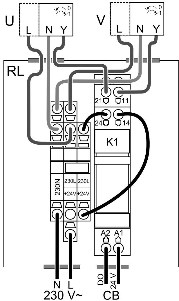
Fig. 1 Damper connection
