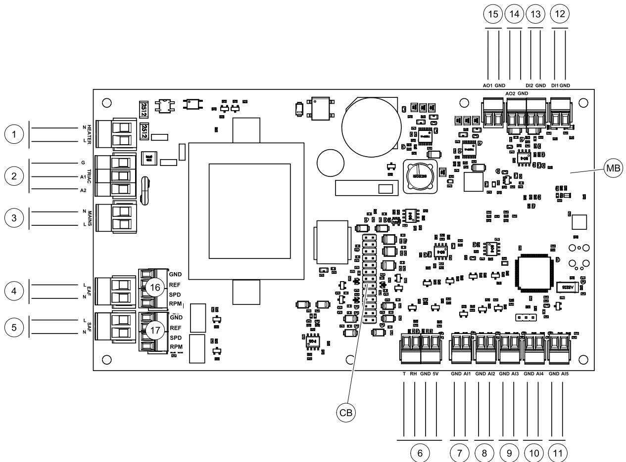
Fig. 5 Main circuit board connections
