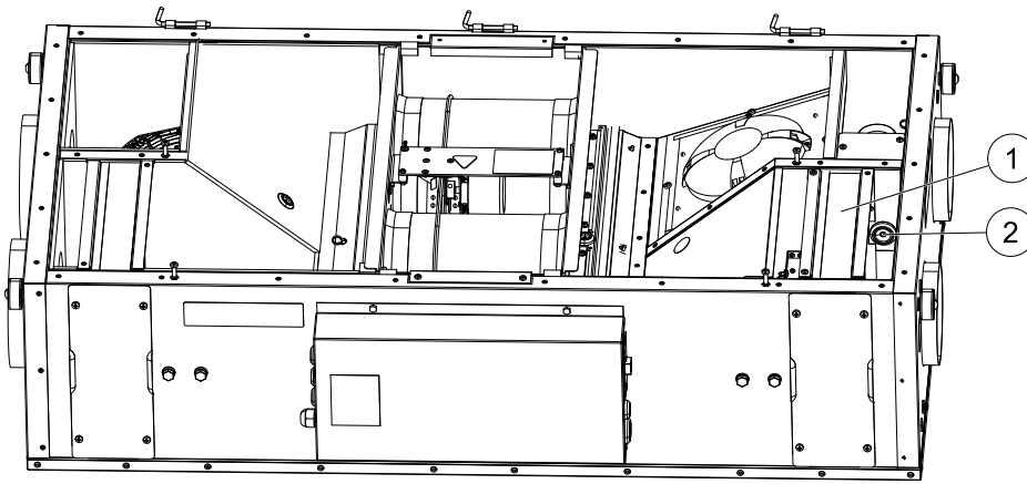
Fig. 11 Overheat protection reset button
