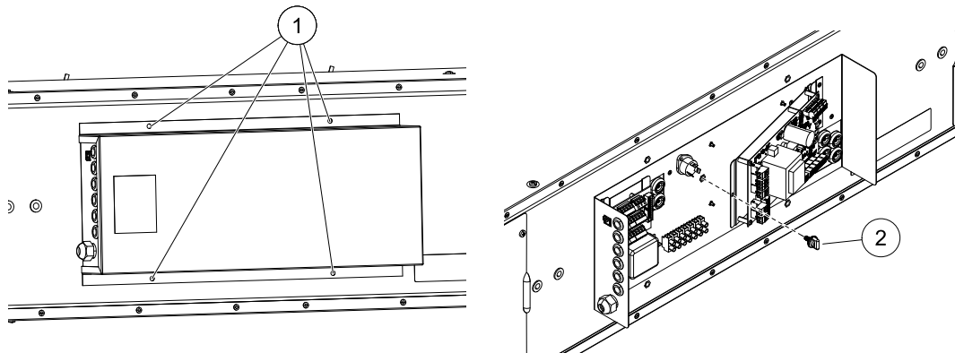
Fig. 4 Print card
