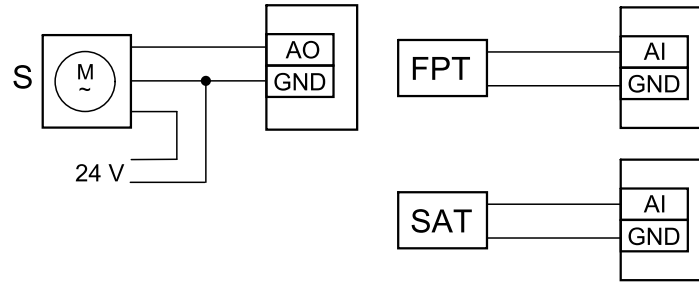
Fig. 15 Water heater connections
