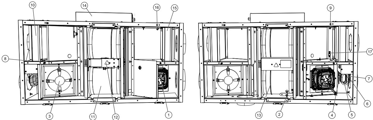
Fig. 10 Internal components
