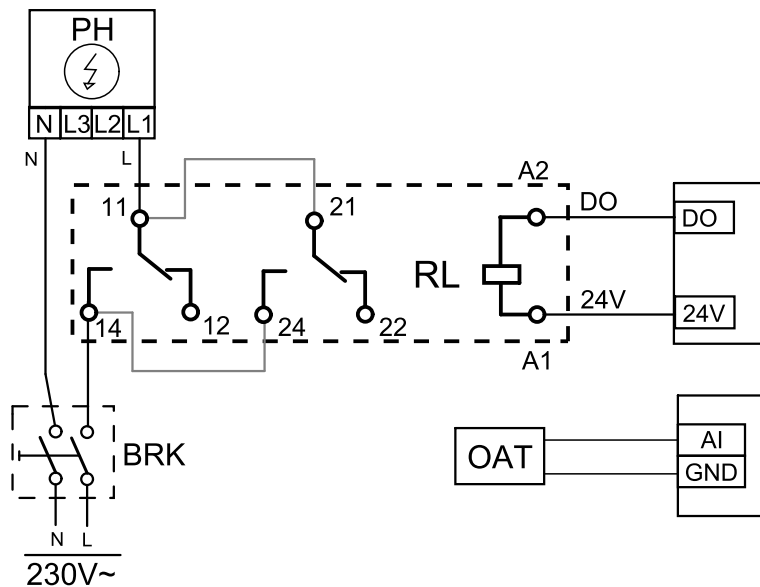
Fig. 14 Pre-heater connections
